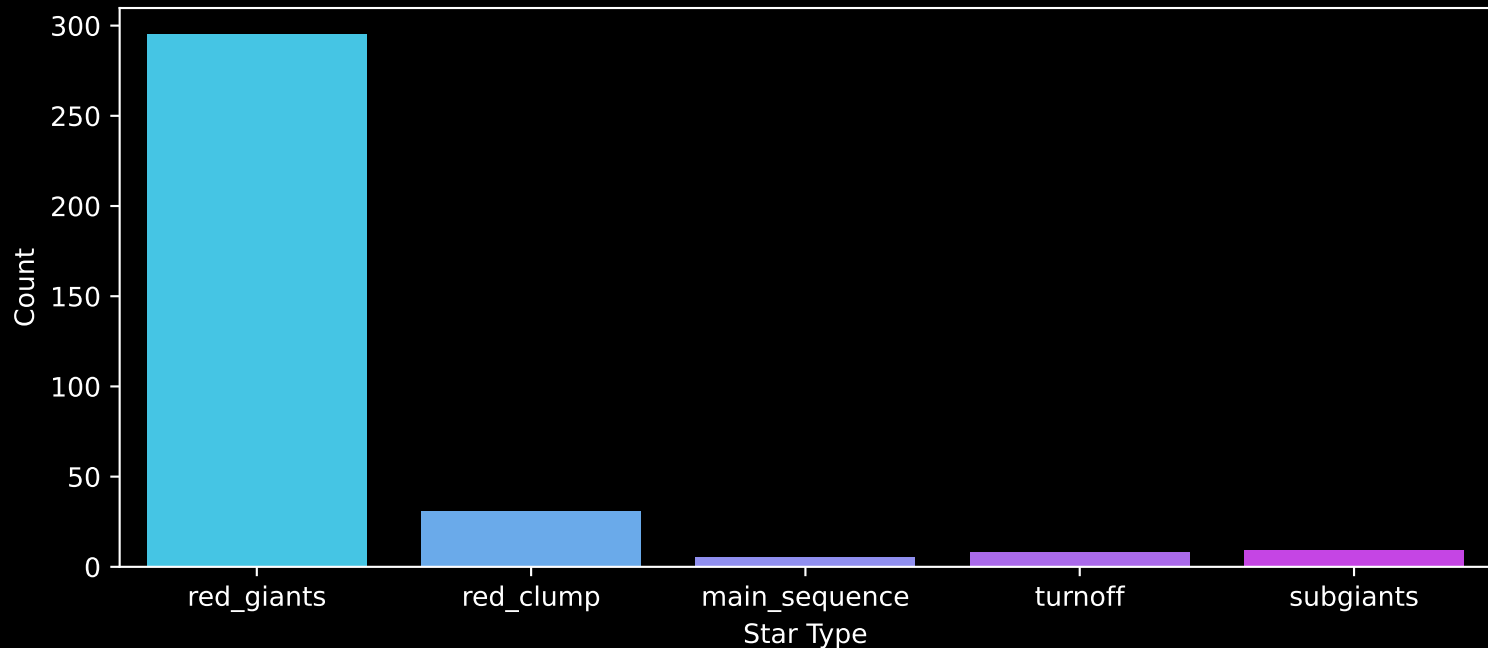
APOGEE DR17 Field: [005+08] Count plot of Star Type
