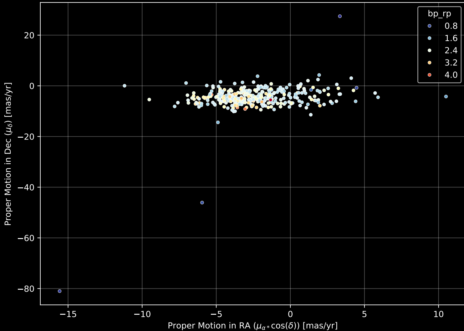
APOGEE DR17 Field: [005+08] Proper Motion Diagram (n= 348)
