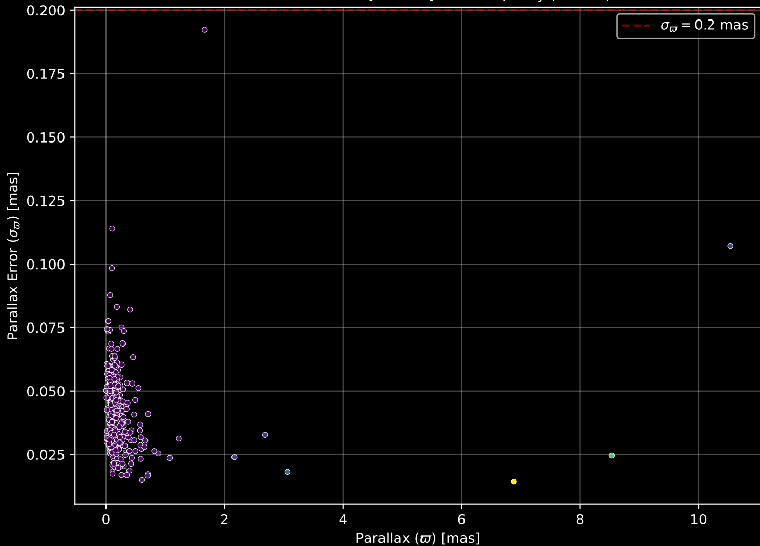
APOGEE DR17 Field: [005+08] Parallax Quality (n= 348)
