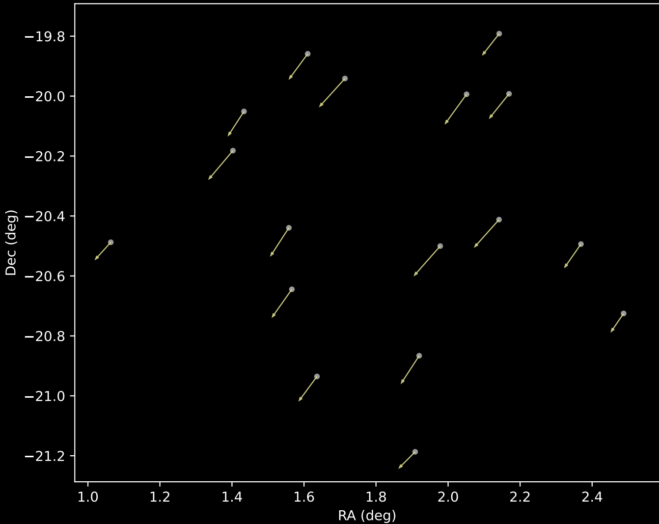
APOGEE DR17 Cluster 17 Proper Motion Vectors (n=17)
