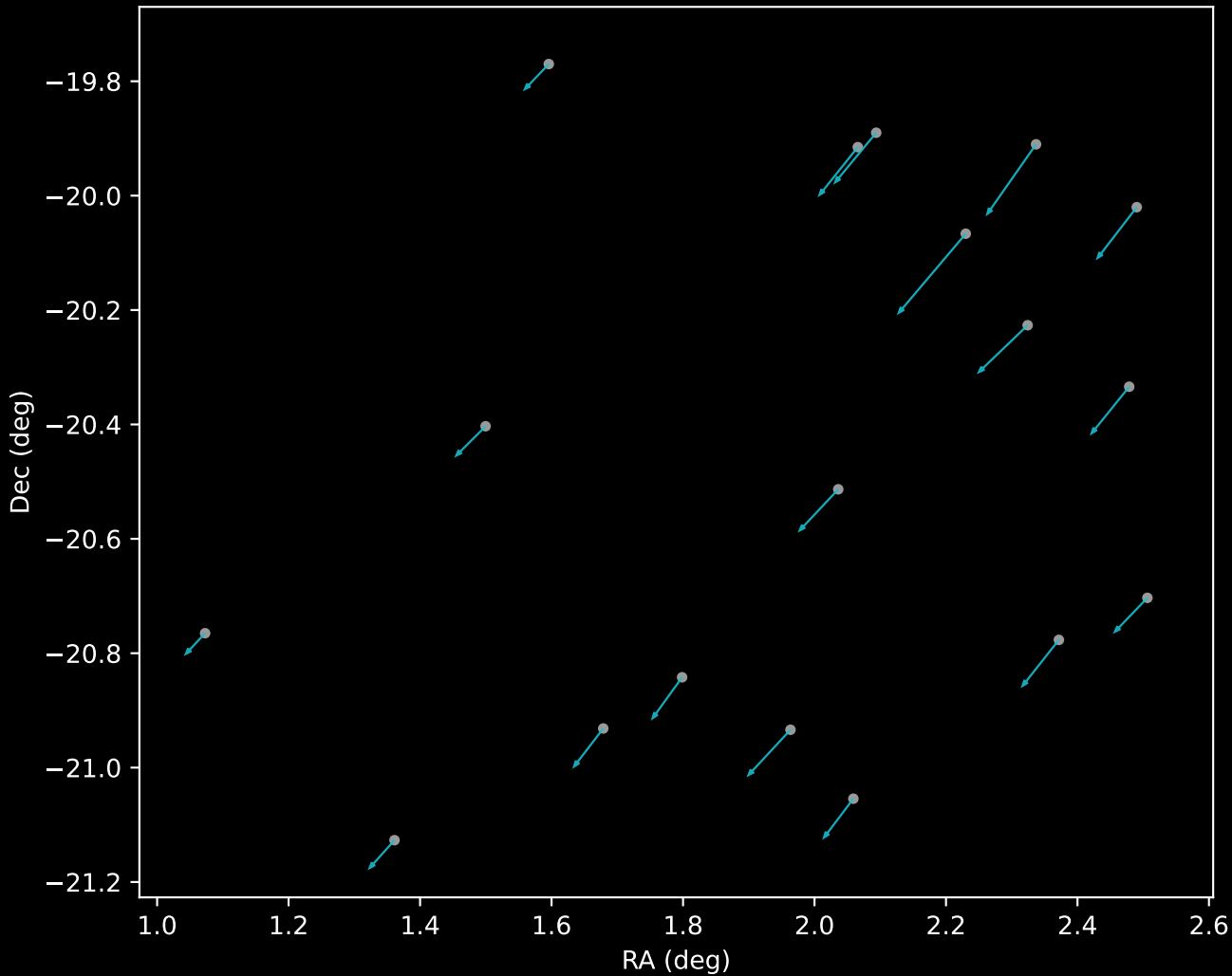
APOGEE DR17 Cluster 18 Proper Motion Vectors (n=18)
