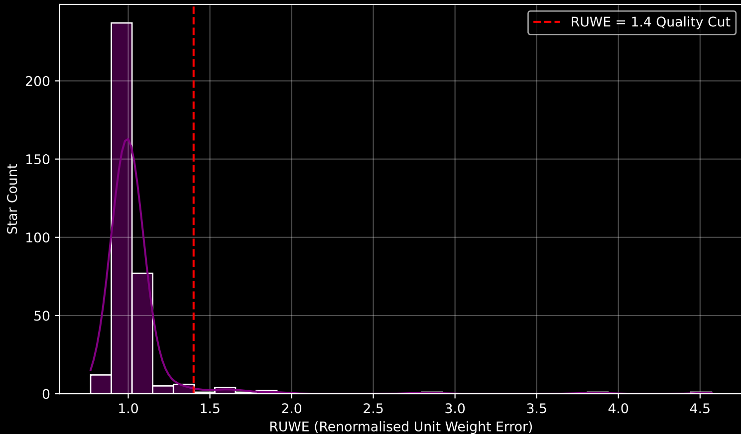
GAPOGEE DR17 Field [005+08] RUWE Distribution (n= 348)
