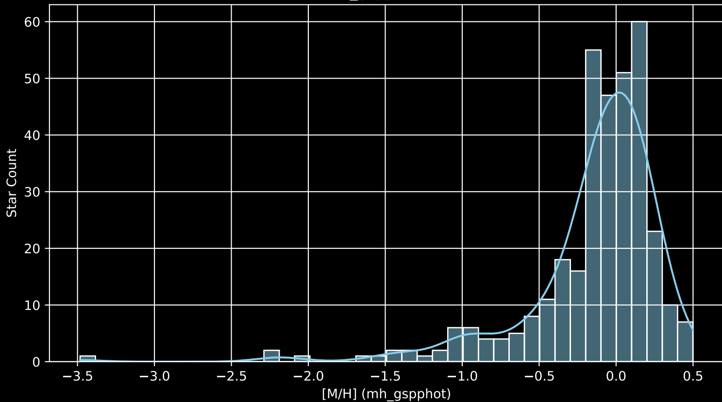
APOGEE DR17 Field: [005+08 [M/H] (mh_gspphot) (n= 344)
